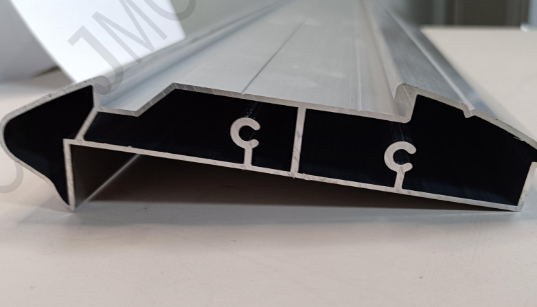
T6063 支撑连接件 Support Connector
