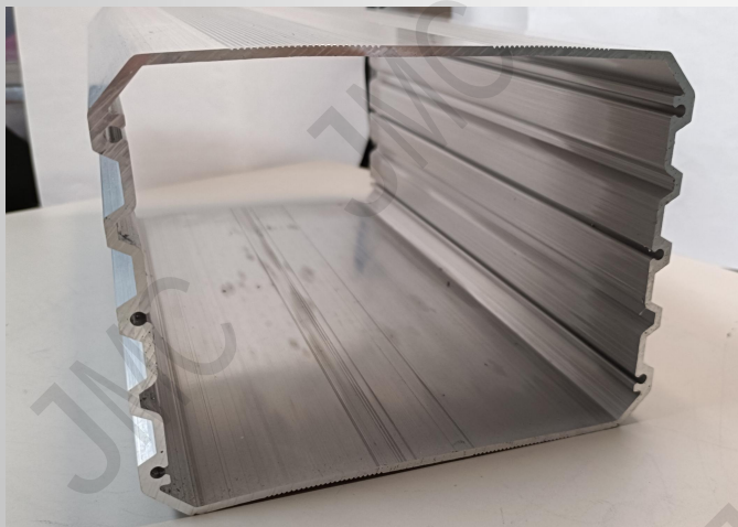
T6063 电池壳 Battery Case
